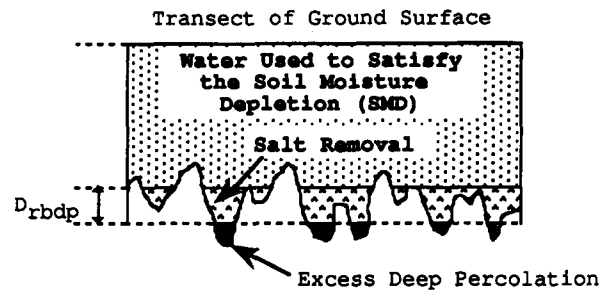
FIG. 5. Deficit Irrigation Nonbeneficial DP
