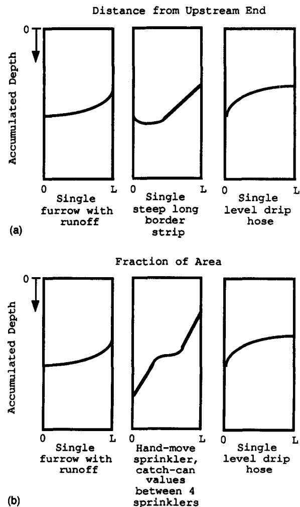
FIG. 12. Typical Variations in Accumulated Water with Location and Arranged by Magnitude: (a) Typical Variation in Local Accumulation of water; Furrow and Border Strip Variations due to Opportunity-Time Differences Only; Drip Variation due to Pressure Variation Only; (b) Typical Variation in Water Accumulated; Values Are Arranged by Magnitude, Rather Than by Location
