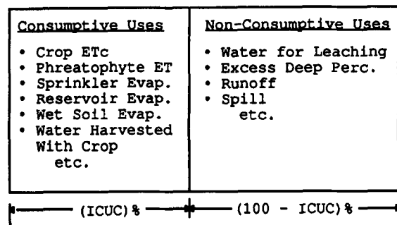
FIG. 9. Irrigation Consumptive Use Coefficient ( ICUC ) Quantifies Division of Irrigation Water into Consumptive and Nonconsumptive Uses
