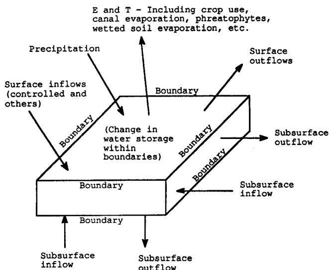
FIG. 2. Components of Simplified Water Balance within Defined Boundaries for Specified Time Interval
