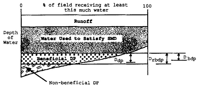
FIG. 7. Irrigation Water Destination Diagram
