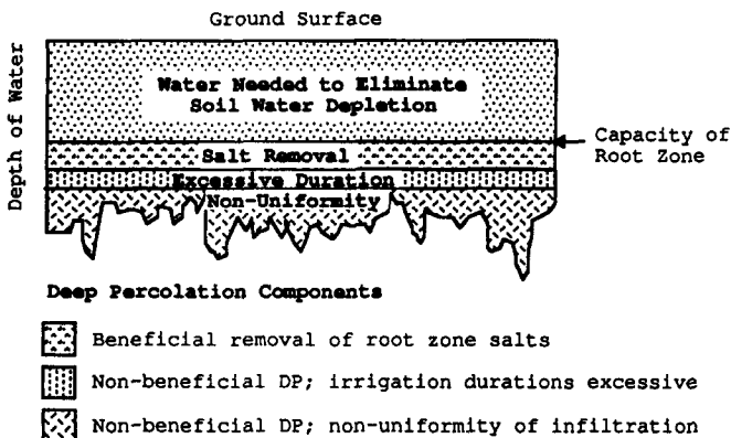
FIG. 4. Overirrigated Field: Beneficial and Nonbeneficial DP
