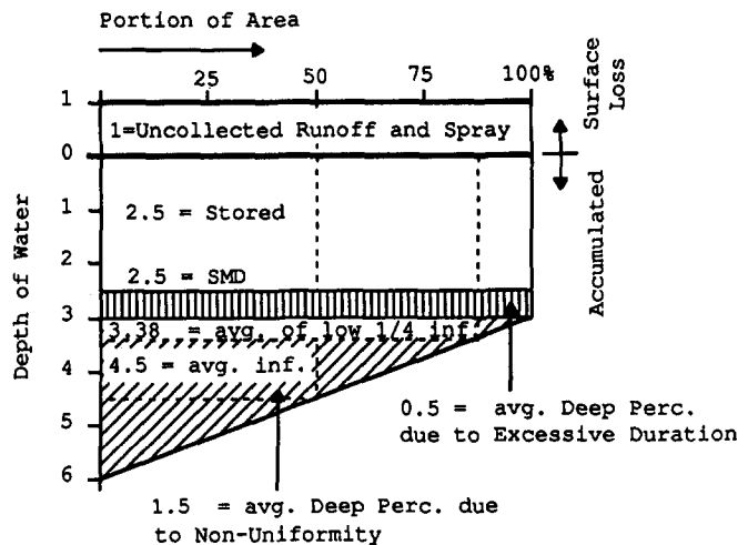
FIG. 16. Overirrigation on All of Field: DU_{iq} = 3.38/4.5 = 0.75 ; AE = 2.5/5.5 \times 100 = 45.5\% ; AD_{iq} = 3.38/3 = 1.13 > 1.0 (Overirrigation)
