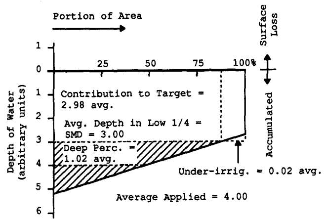
FIG. 14. Simplified Case of "Perfect" Irrigation Scheduling: DU_{iq} = 0.75 ; field AE = 74.5\%
