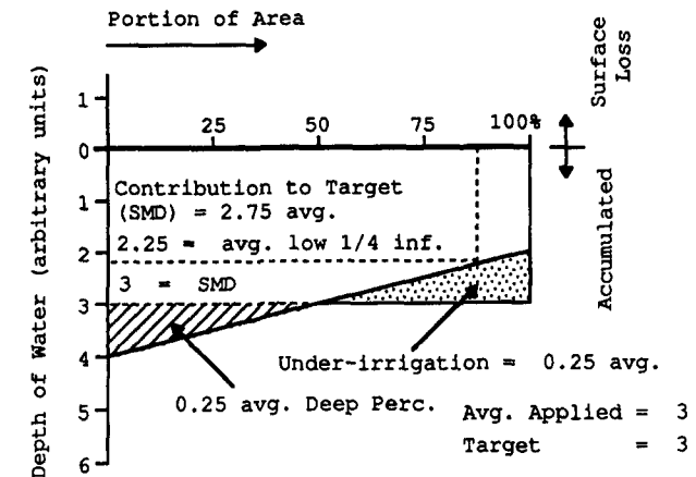
FIG. 15. Water Destination Diagram with Average Accumulated Depth Equal to Target Depth (3 Units) and No Surface Losses: DU_{iq} = 2.25/3 = 0.75 ; AD_{iq} = 0.75 (Underirrigation)
