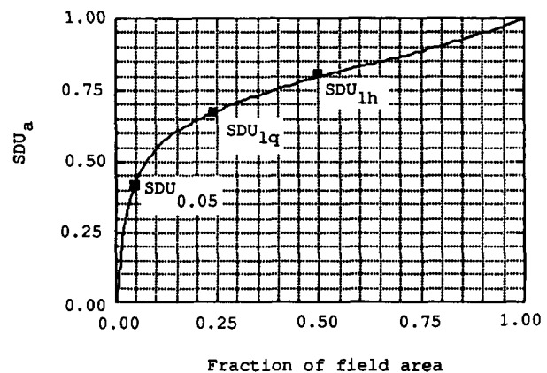
FIG. 13. Relationship between SDU_a and Defining Fraction of Field Area Having Lowest Depths in Distribution (Values Normally Distributed with CV = 0.25 )
